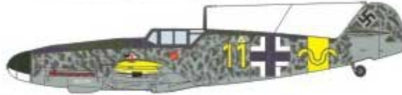
Bf-109G-2R6 "Yellow 11", pilot Oblt. Hermann Graf, 9/JG 52, Pflanzk, Rusia, September 1942.
