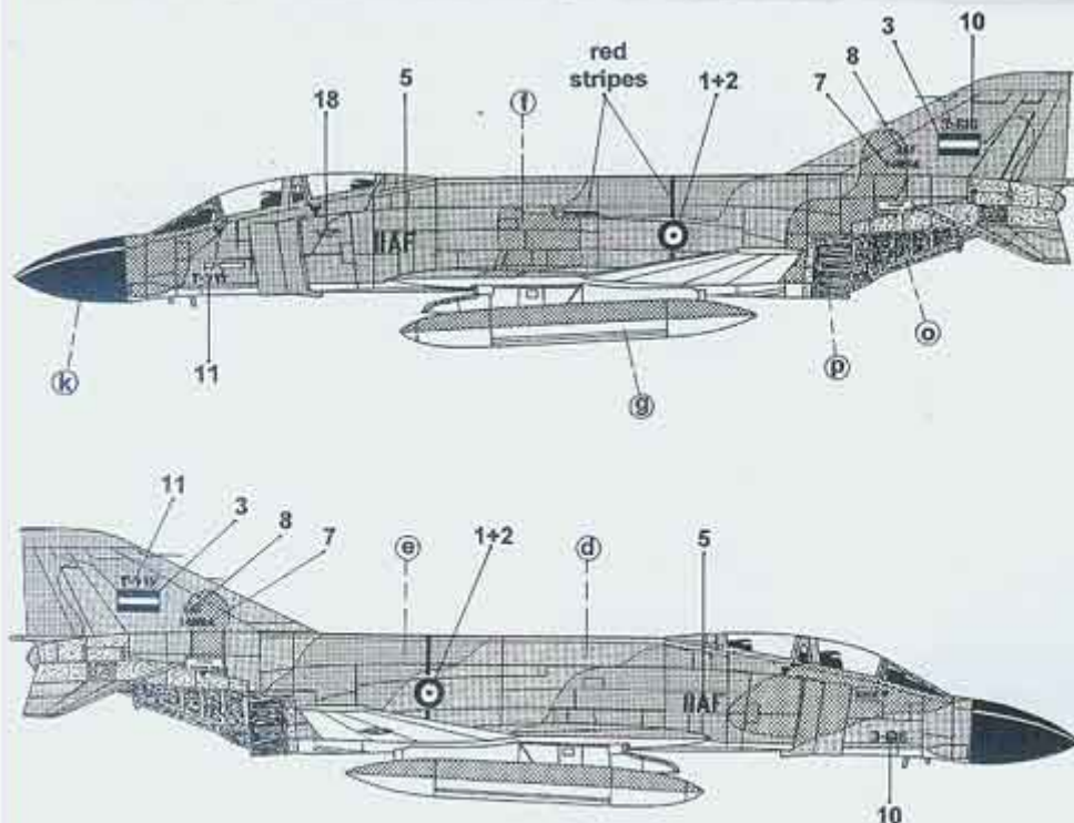
2 F-4D 67-14884 / 3-616, 308 th TFS, 32 nd TFW, Imperial Iranian Air Force (IIAF). TFB.3 Nojeh, 1973.
