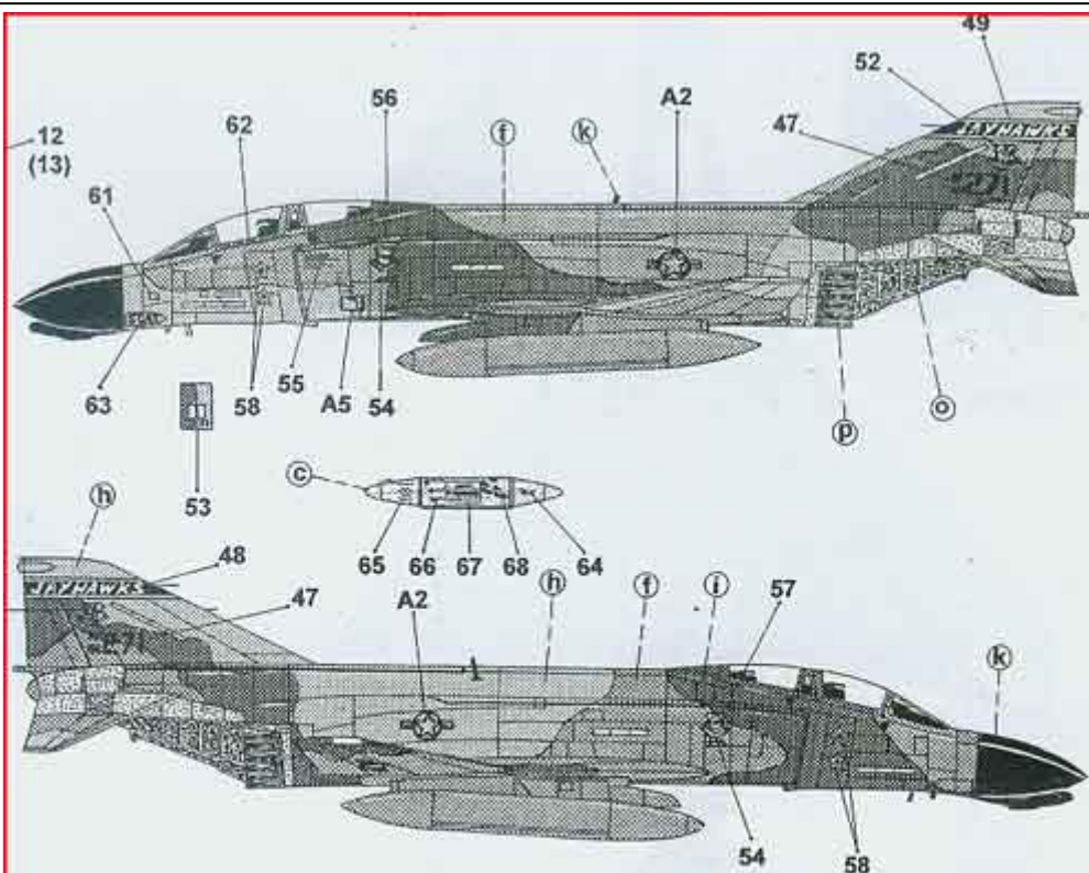
6 F-4D 66-0271 127 th TFS, 184 TFG, Kansas ANG. McConnell AFB, Wichita, Kansas, 1986
