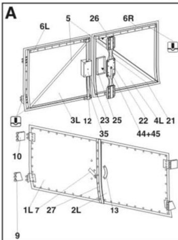
Mittlere Zugkraftwagen 8t Sd.Kfz.7 Doors of the storage compartment P35-218
