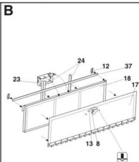
Mittlere Zugkraftwagen 8t Sd.Kfz.7 Doors of the storage compartment P35-218
