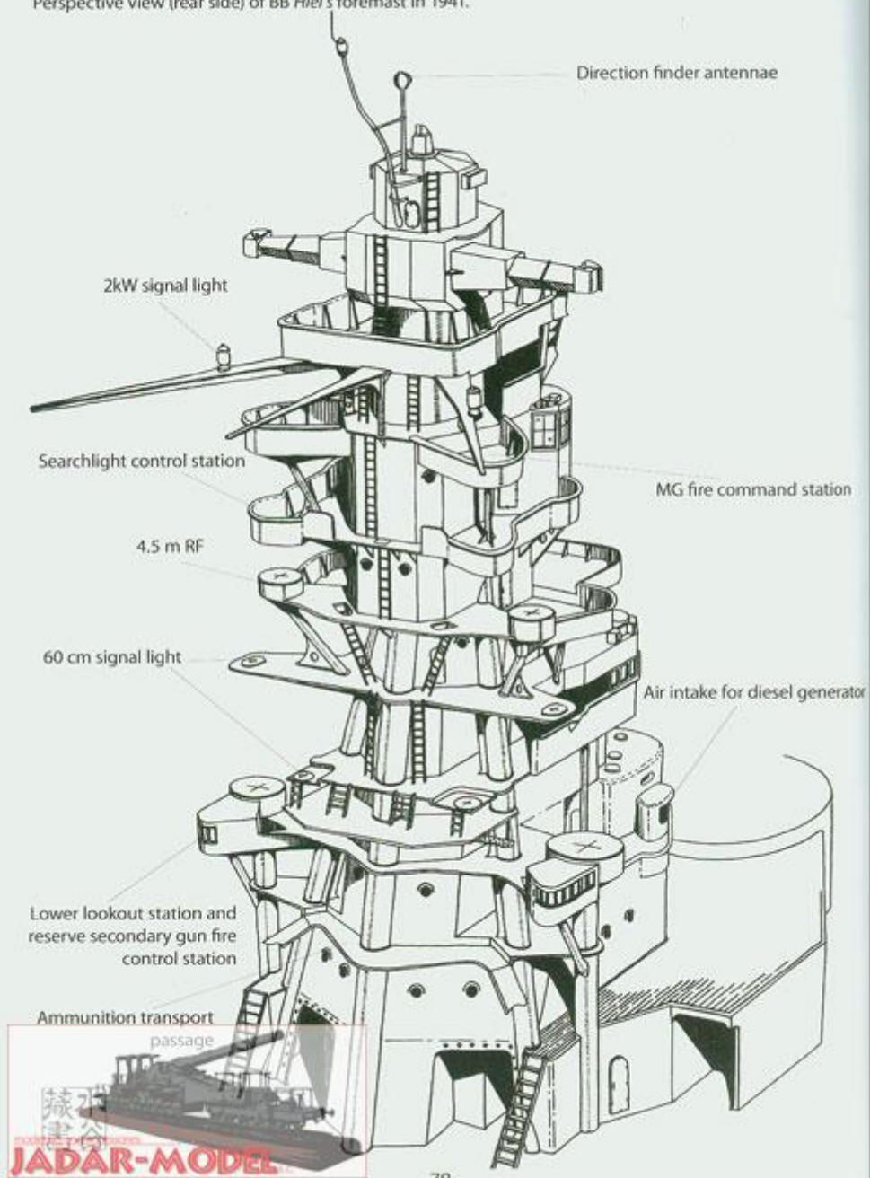
Figure 71 Perspective view (rear side) of BB Hiei 's foremast in 1941.
