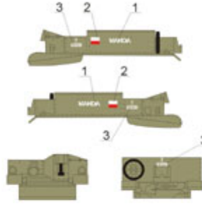
[K] Universal Carrier mk I, Poziom pancerny '10', 1940. Universal Carrier mk I '10' armoured train, 1940.
