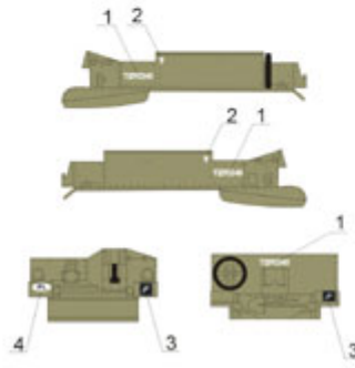
[K] Universal Carrier mk II, 13 Puk Dragonów, 1 Dywizja Pancerna, Holandia, 1944. Universal Carrier mk II, 13th Dragoons Regiment, 1st Armoured Division, Holland, 1944.
