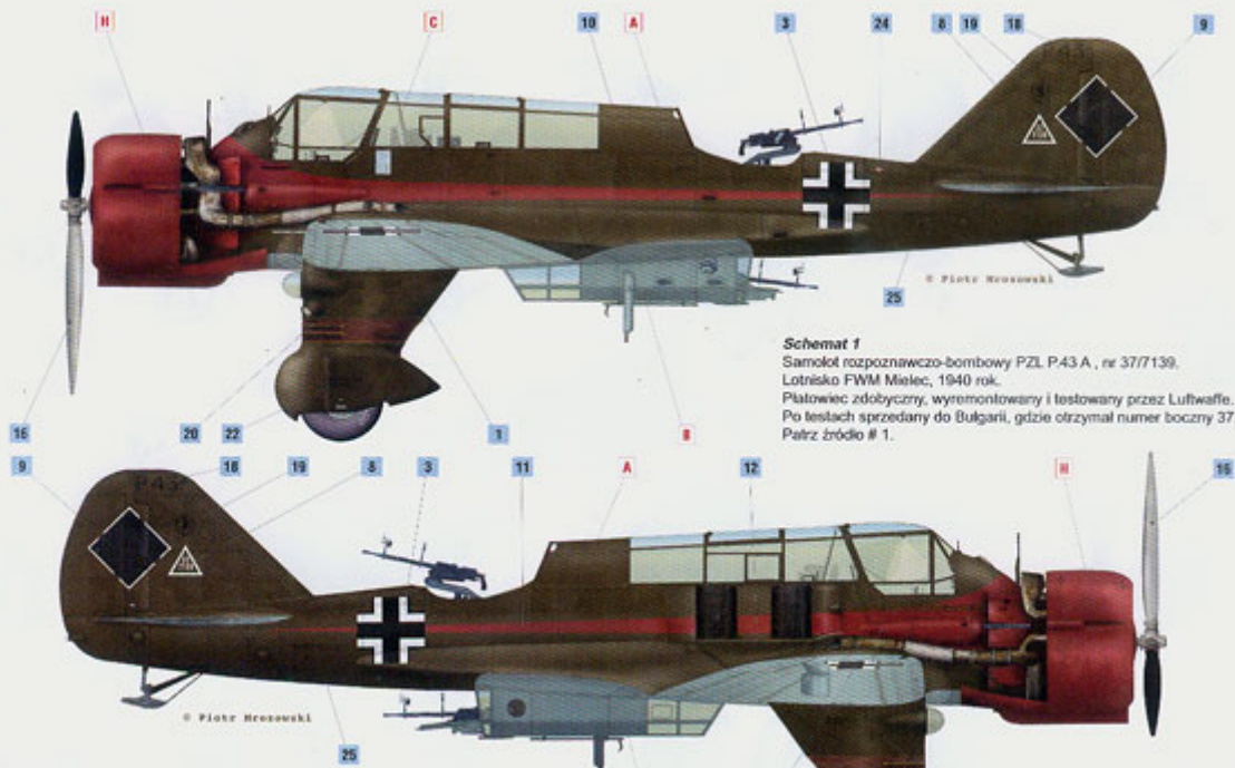
Scheme 1 Reconnaissance-bomber aircraft PZL P.43 A, No. 37/7139. Airfield FWM Mielec, 1940. Airframe captured, repaired and tested by the Luftwaffe. After the tests sold to Bulgaria, where received a side number "37" See source # 1
