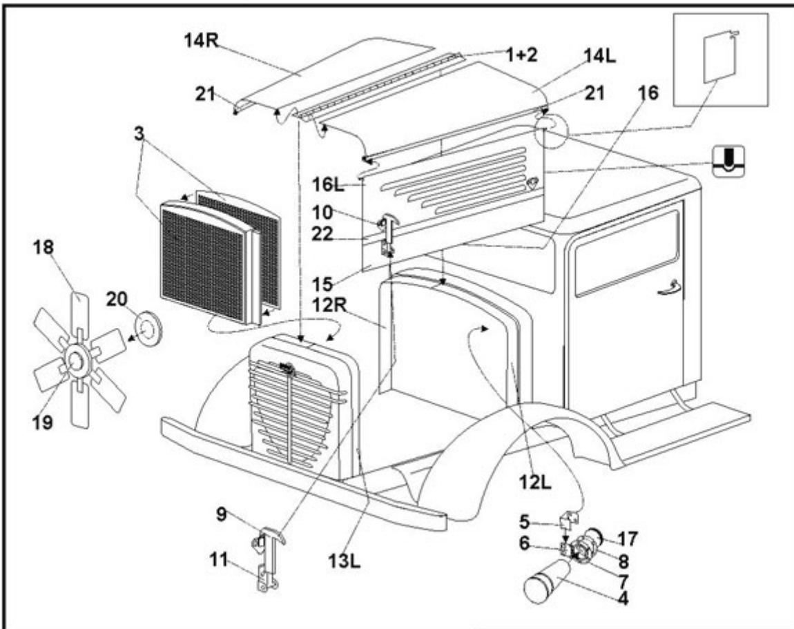
BUSSING-NAG 500 A ENGINE HOOD
