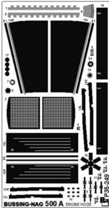
BUSSING-NAG 500 A ENGINE HOOD
