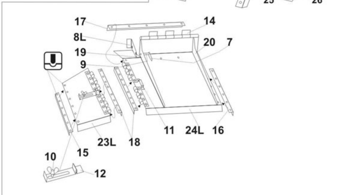
Pz.Kpfw.VI TIGER B front and back fenders
