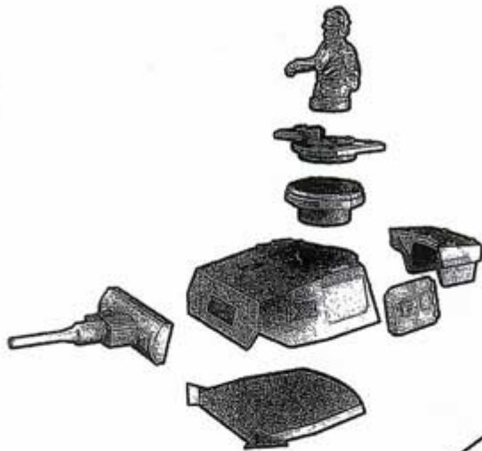
1. Turret sub-assembly
