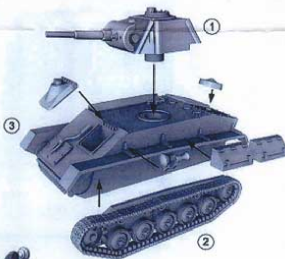
4. General Assembly.
