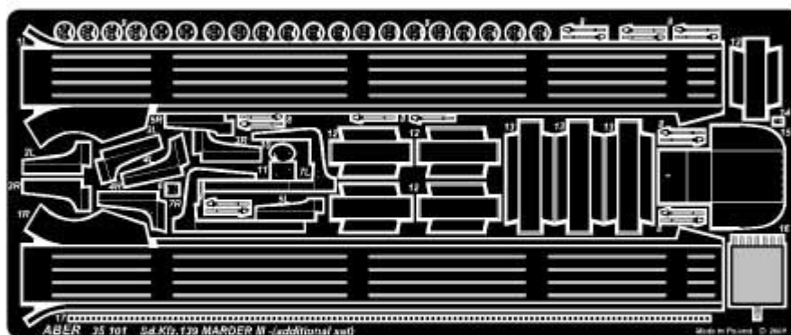
35 101 Sd.Kfz. 139 "Marder III" (Additional set) (TAMIYA model)
