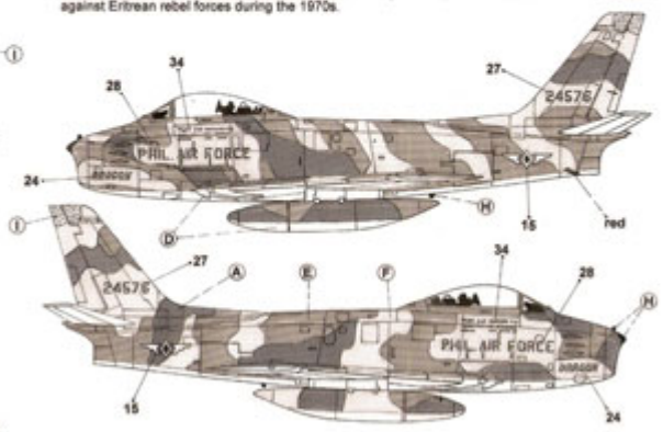
4 F-86F-30 52-4576 "DRAGON" – 9 th TFS, 6 th TFW, Philippine Air Force, Edwin Andrews AB, Zamboanga, Mindanao, 1974. Philippine Sabres were used in the COIN role against MNLF rebel forces during the fighting in Mindanao. Several F-86Fs from the 9 th TFS received this camouflage scheme during in 1973. The applied paints degenerated under the hard tropical conditions and heavy chipping appeared quickly "DRAGON" was lost due to ground fire during 1974.
