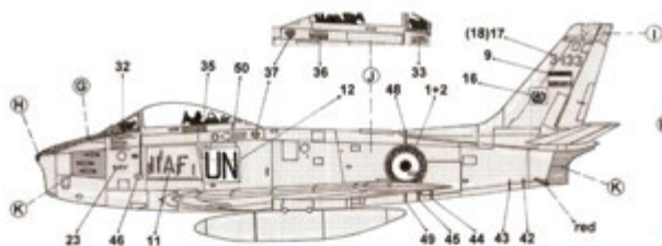
1 F-86F-25 51-13244 / 3-133 – 103 rd TFS, Imperial Iranian Air Force, Kamina AB, Congo, 1963. The IIAF received the first of 52 F-86F Sabres, updated with the F-40 slatted wings and 4 underwing hardpoints, in 1960. Normally based at 1 TFB Mehrabad, 3-133 was one of four IIAF Sabres operating out of Kamina AB, between January and May 1963, as part of the United Nations Fighter Wing during the Katanga crisis. The IIAF F-86Es were very active, flying more operational sorties than the co-based Swedish and Philippine contingents combined, one of the Sabres suffering damage due to ground fire.
