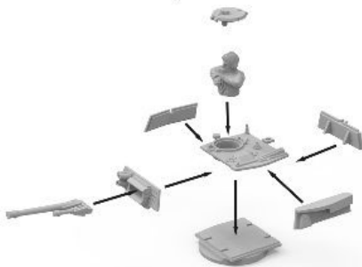
5. MK2 turret assembly
