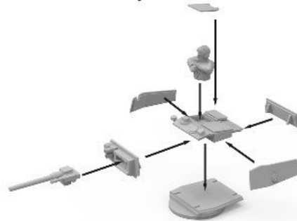
6. MK4 turret assembly
