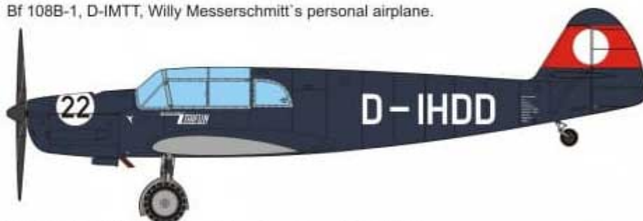
Bf 108B-1, D-IHDD , in Isle of Man air rally markings, 1937.
