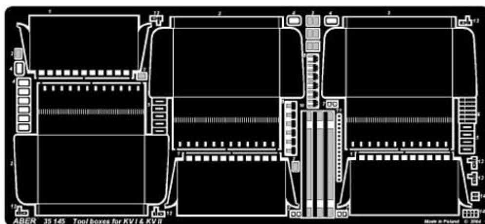
35 145 Russian Heavy Tank KV-I or KV-II, Vol.3 - additional set - Tool Boxes for early fenders (TAMIYA model)
