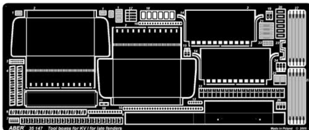
35 147 Russian Heavy Tank KV-I, Vol.5 - additional set - Tool Boxes for late fenders (TAMIYA model)
